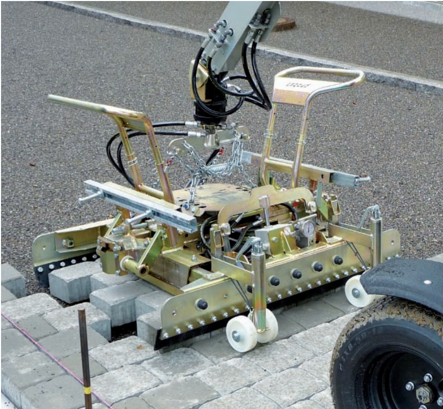
HVZ herring bone 45° - the ideal solution for bigger areas of herring bone pattern. This type of clamp handles 45° packed layers of stones and allows an installation without filling gaps by adding stones.
